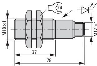
LSO-R18S-B2000-PD
